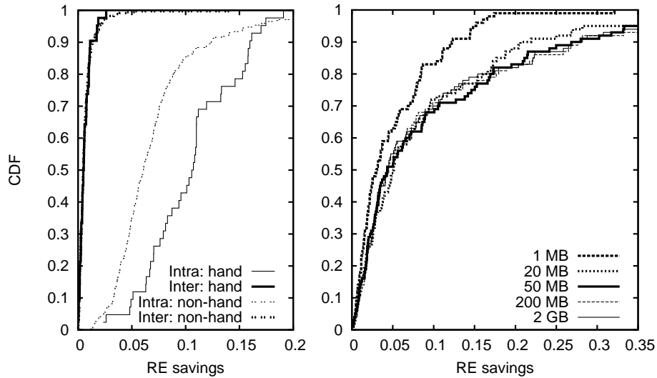
(a) Average intrauser and interuser redundancy across multiple traces (b) Intrauser redundancy across top 100 (by bytes) handholds for varying dictionary sizes
